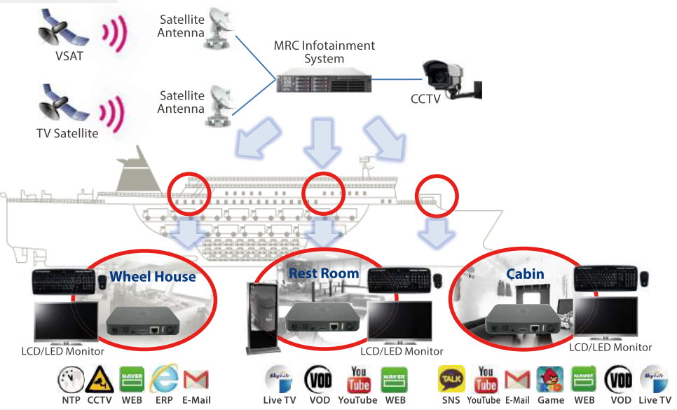
Wiring Diagram of MRC Infotainment System
