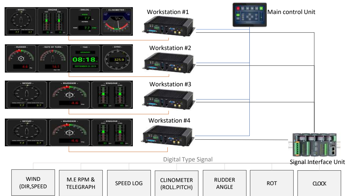
System Configuration
