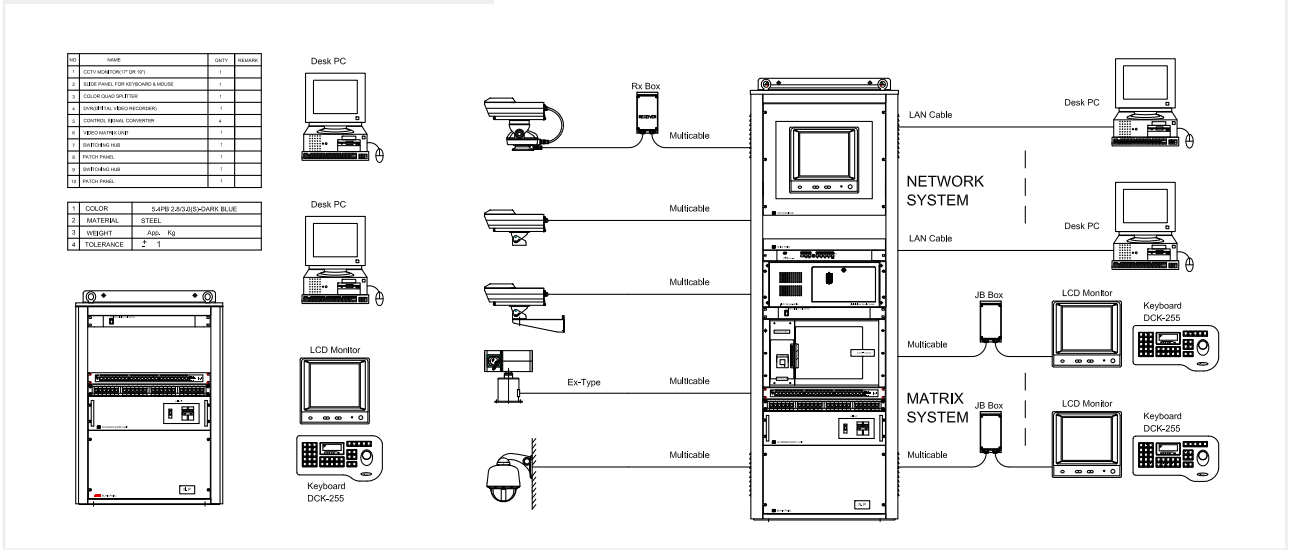
Wiring Diagram of CCTV System LAN[P] or Analog Type
